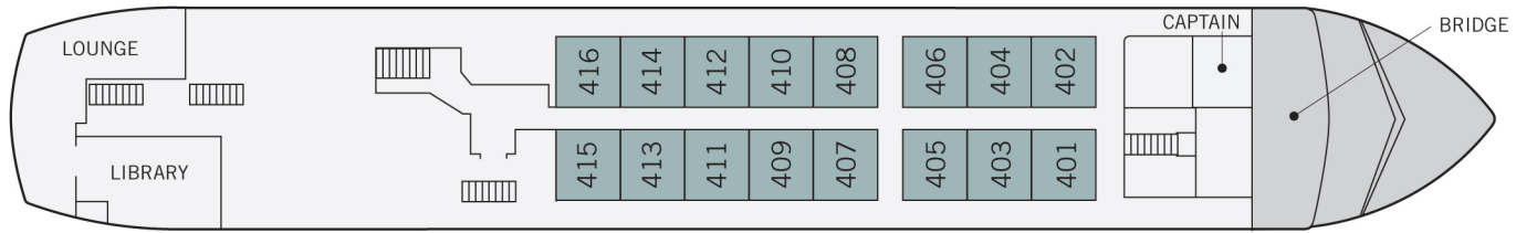
BRIDGE DECK
